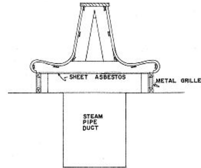
SETTEE SECTION SCALE 3/4" = 1'-0"
