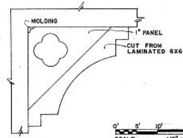
CORNICE DETAIL SCALE 1 1/2" = 1'-0"
