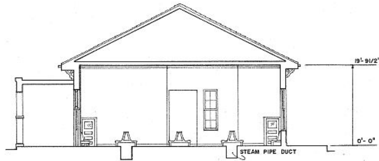
SECTION B SCALE 1/8" = 1'-0"
